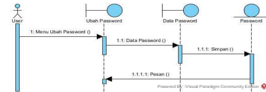
Gambar 3. 30 Sequence Diagram Ubah Password User
