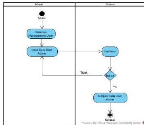
Gambar 3. 13 Activity Diagram Managemen User Admin
